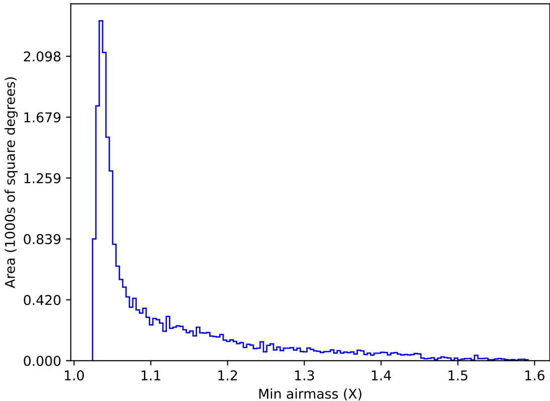
ddf_acor_sf30_lsf40_lsr10_v3.4_10yrs All sky u band: Min airmass
