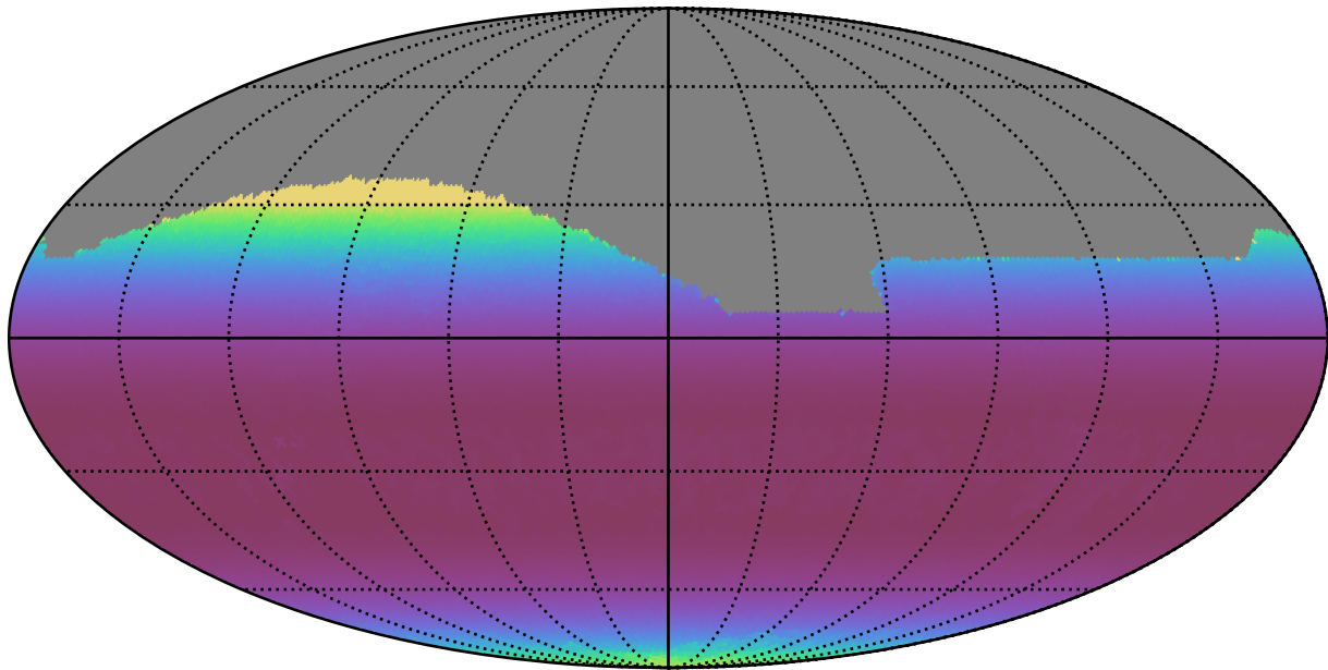
ddf_acor_sf30_lsf40_lsr10_v3.4_10yrs All sky r band: Min airmass
