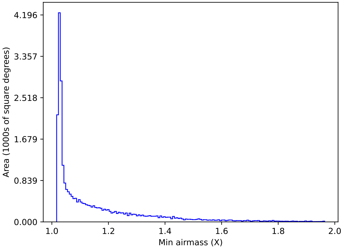
ddf_acor_sf30_lsf40_lsr10_v3.4_10yrs All sky r band: Min airmass
