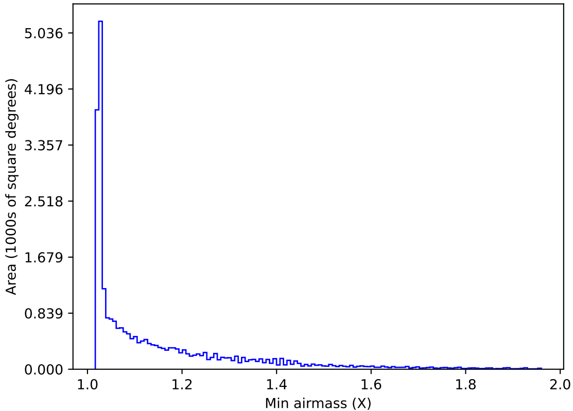
ddf_acor_sf30_lsf40_lsr10_v3.4_10yrs All sky all bands: Min airmass
