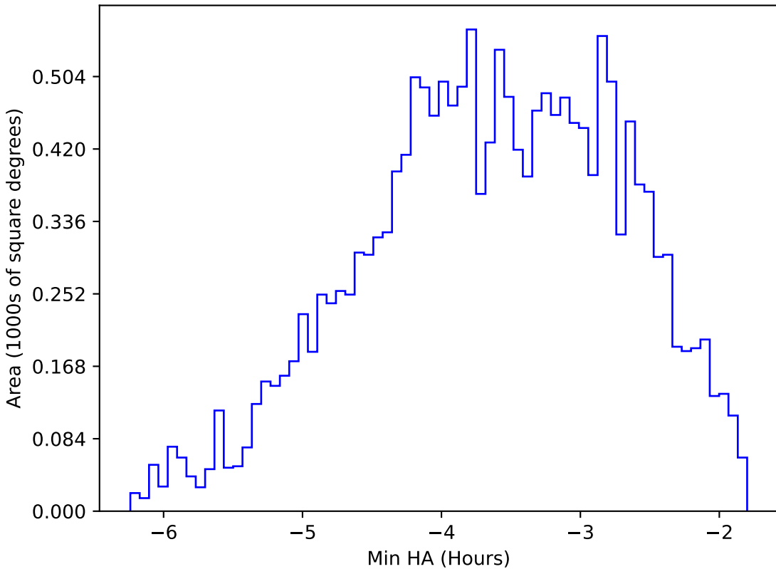
ddf_acor_sf30_lsf40_lsr10_v3.4_10yrs WFD y band: Min HA
