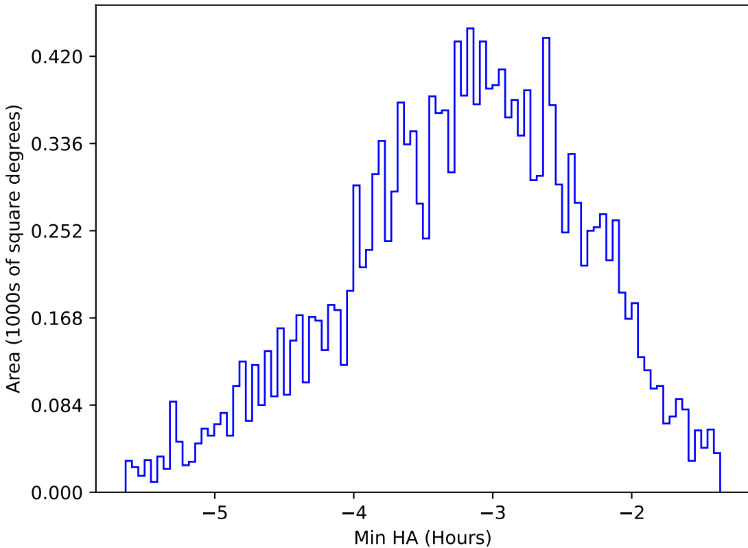
ddf_acor_sf30_lsf40_lsr10_v3.4_10yrs WFD u band: Min HA
