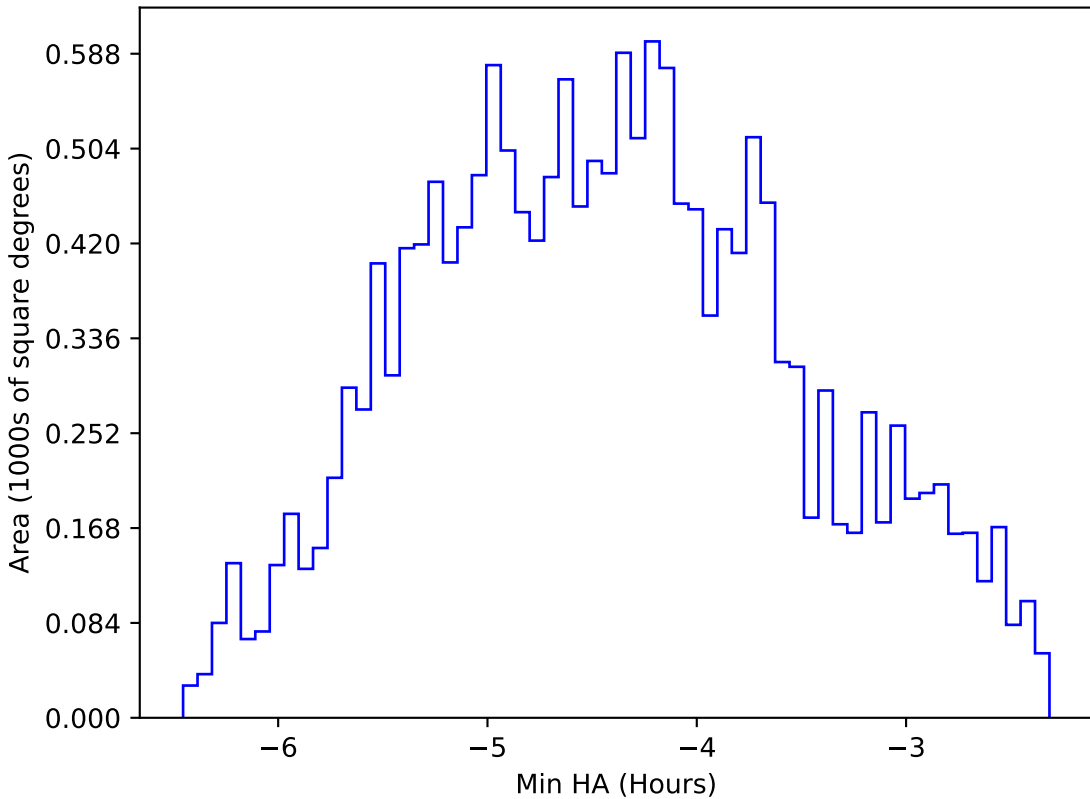
ddf_acor_sf30_lsf40_lsr10_v3.4_10yrs WFD r band: Min HA
