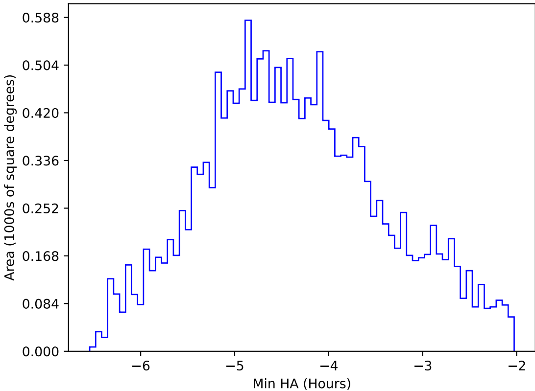
ddf_acor_sf30_lsf40_lsr10_v3.4_10yrs WFD i band: Min HA
