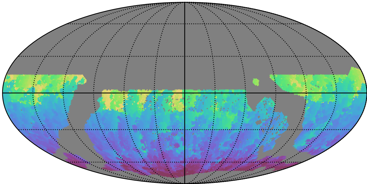
ddf_acor_sf30_lsf40_lsr10_v3.4_10yrs WFD g band: Min HA
