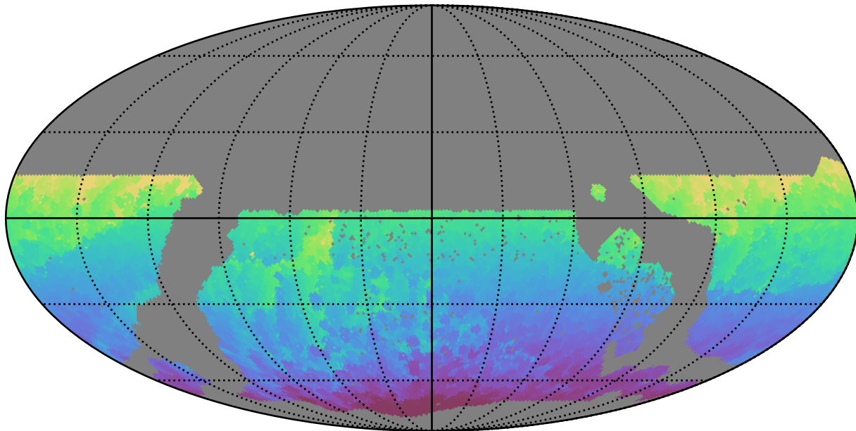
ddf_acor_sf30_lsf40_lsr10_v3.4_10yrs WFD all bands: Min HA
