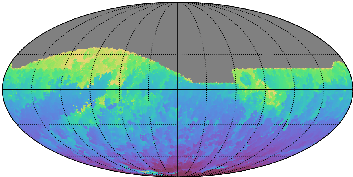
ddf_acor_sf30_lsf40_lsr10_v3.4_10yrs All sky z band: Min HA
