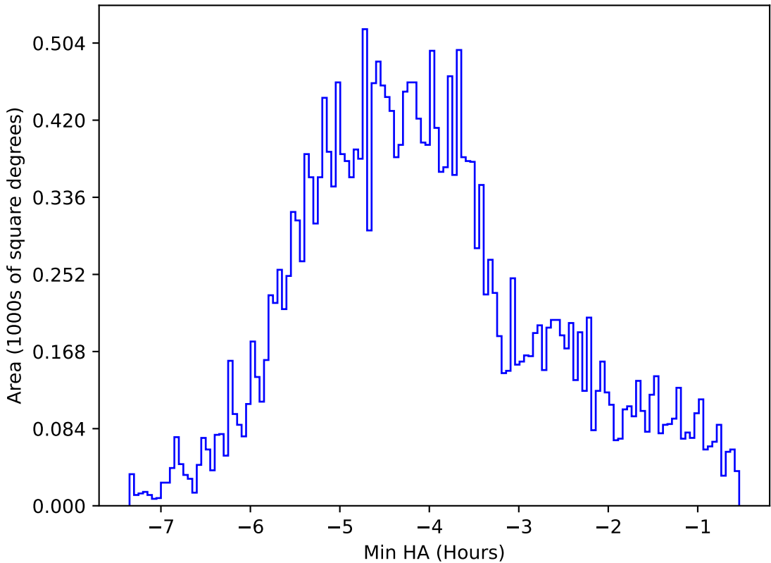
ddf_acor_sf30_lsf40_lsr10_v3.4_10yrs All sky z band: Min HA
