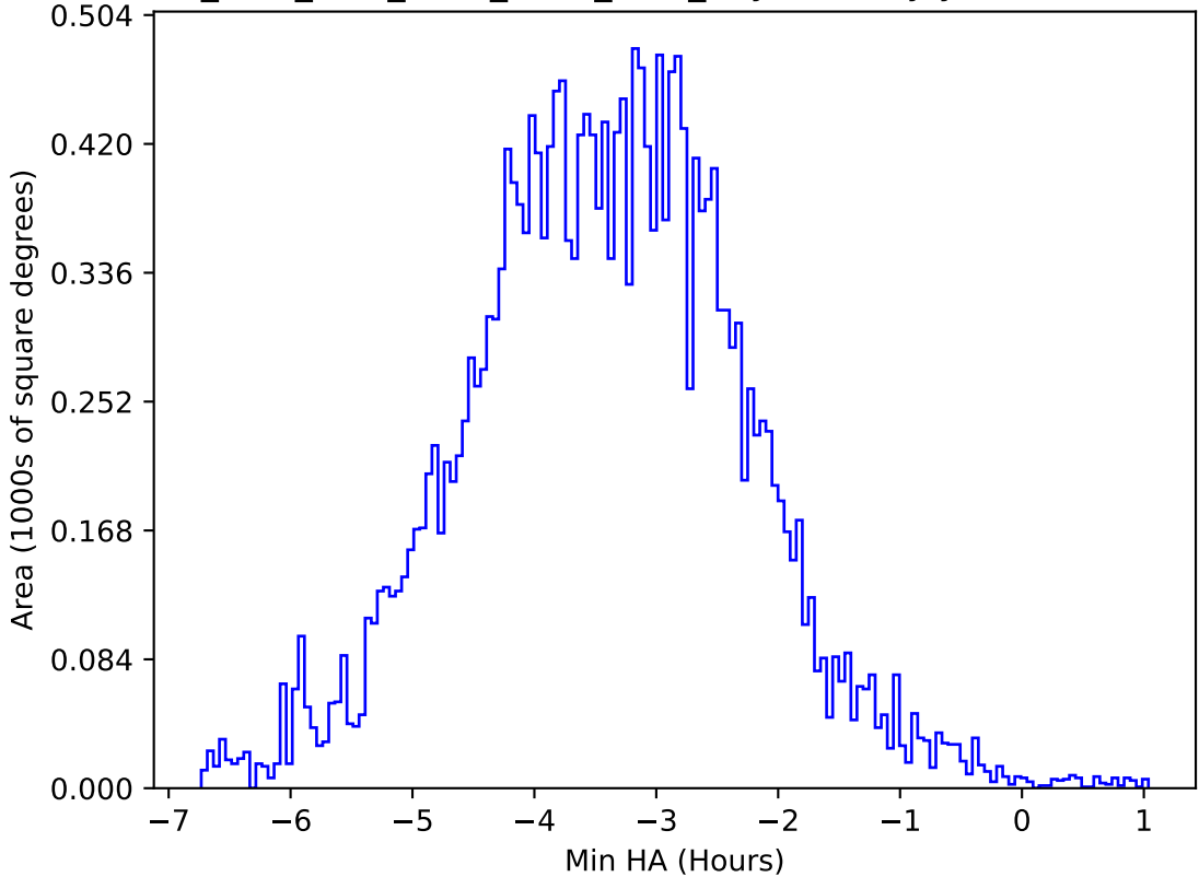
ddf_acor_sf30_ls40_lsr10_v3.4_10yrs All sky y band: Min HA
