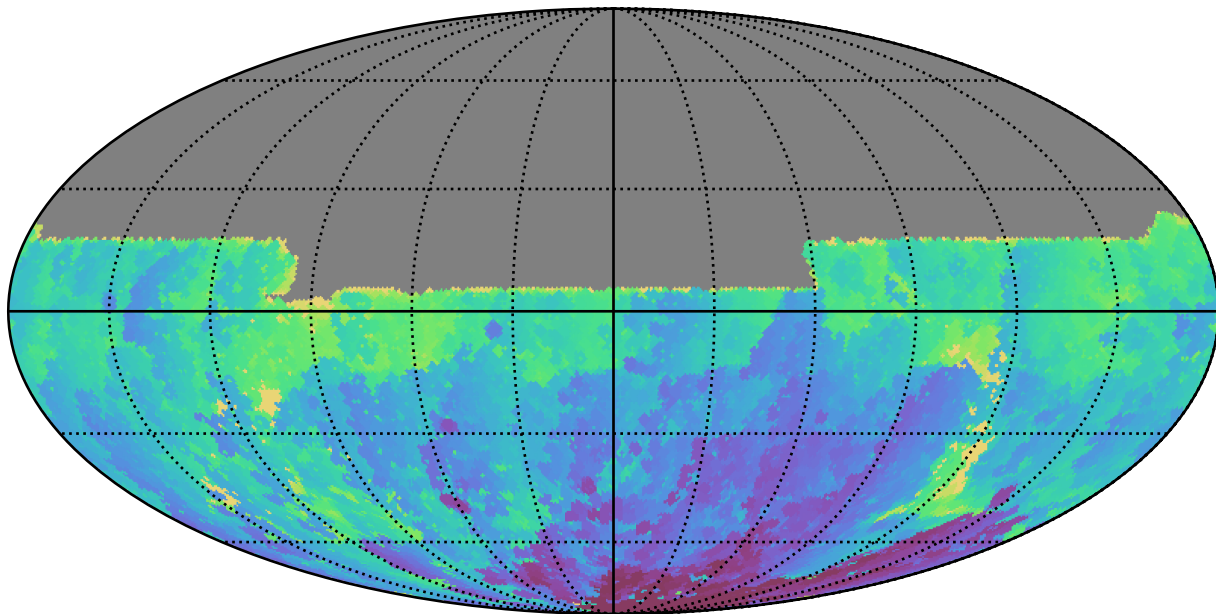
ddf_acor_sf30_lsf40_lsr10_v3.4_10yrs All sky u band: Min HA
