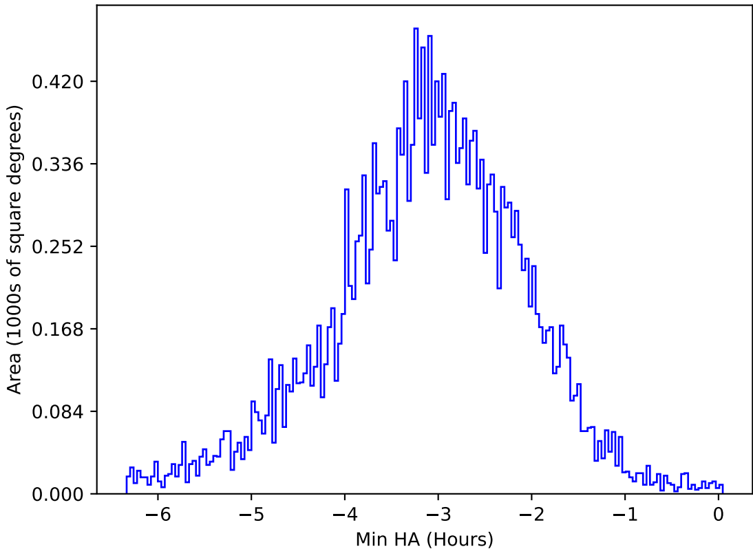
ddf_acor_sf30_lsf40_lsr10_v3.4_10yrs All sky u band: Min HA
