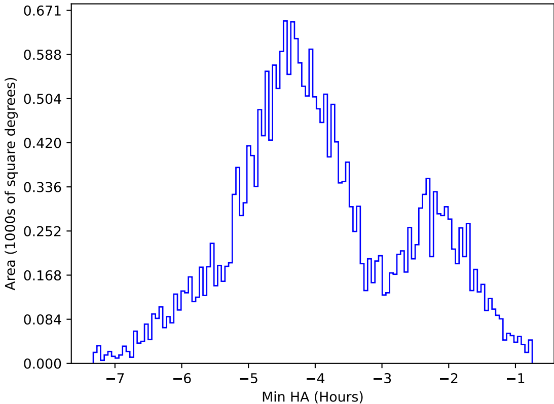
ddf_acor_sf30_lsf40_lsr10_v3.4_10yrs All sky g band: Min HA
