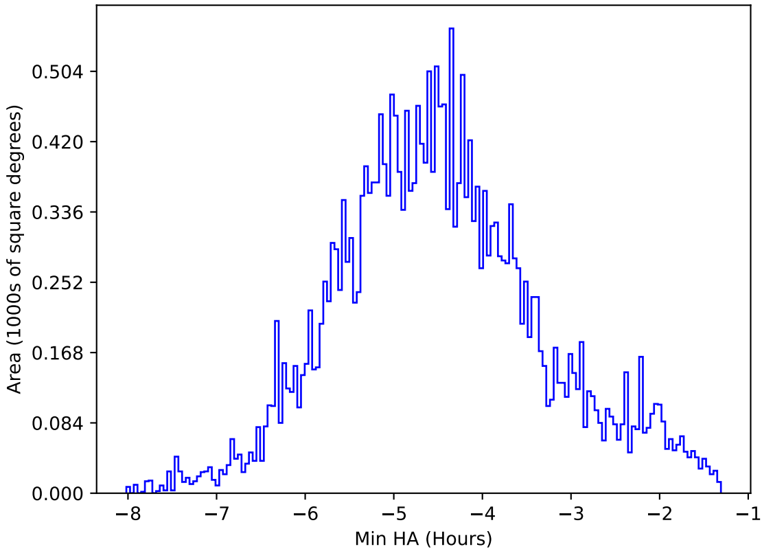
ddf_acor_sf30_lsf40_lsr10_v3.4_10yrs All sky all bands: Min HA
