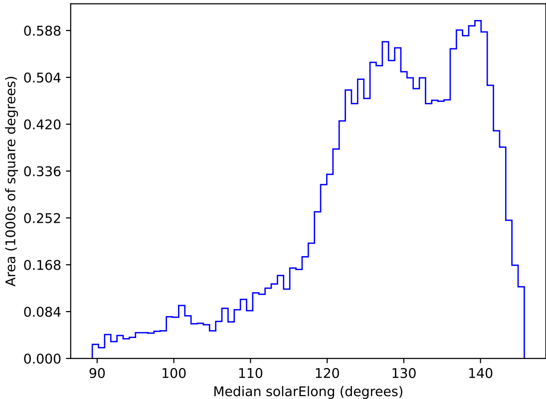
ddf_acor_sf30_lsf40_lsr10_v3.4_10yrs WFD z band: Median solarElong
