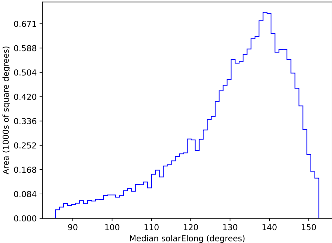
ddf_acor_sf30_lsf40_lsr10_v3.4_10yrs WFD u band: Median solarElong
