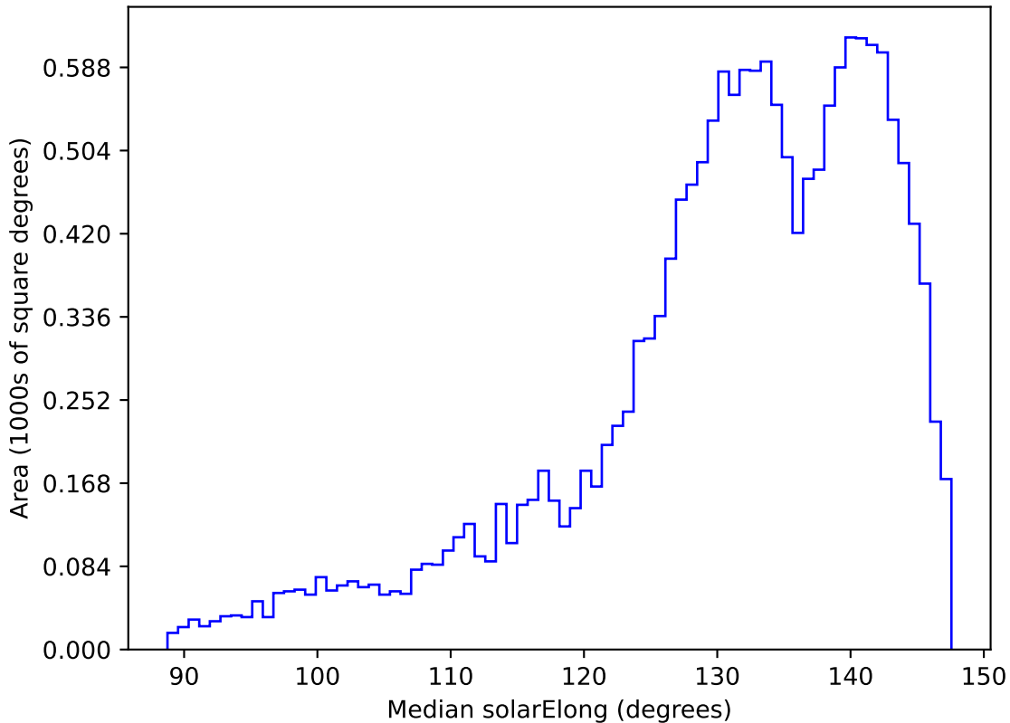
ddf_acor_sf30_lsf40_lsr10_v3.4_10yrs WFD r band: Median solarElong
