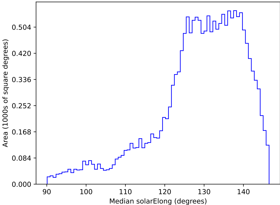
ddf_acor_sf30_lsf40_lsr10_v3.4_10yrs WFD i band: Median solarElong
