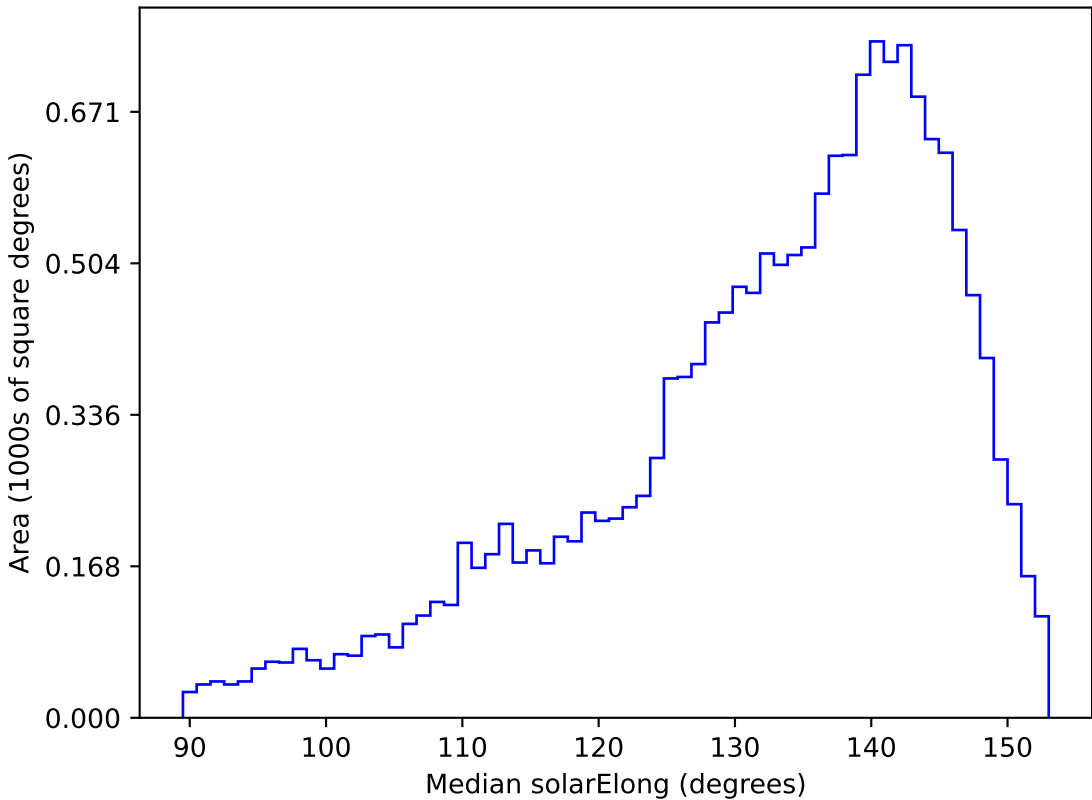
ddf_acor_sf30_lsf40_lsr10_v3.4_10yrs WFD g band: Median solarElong
