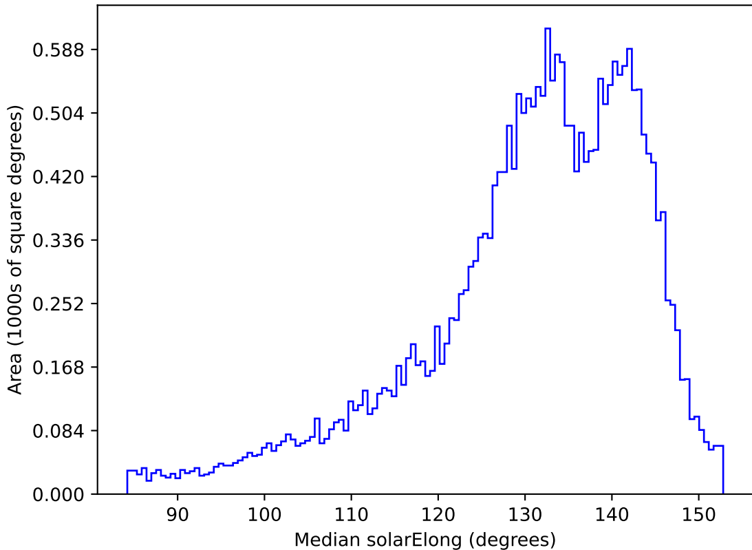
ddf_acor_sf30_lsf40_lsr10_v3.4_10yrs All sky r band: Median solarElong
