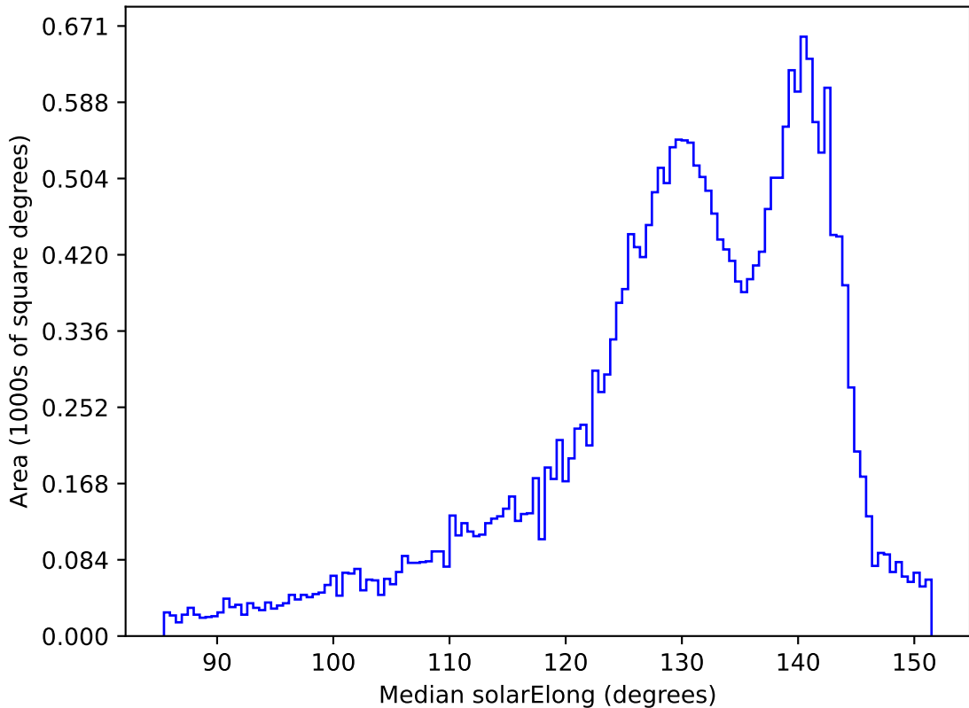
ddf_acor_sf30_lsf40_lsr10_v3.4_10yrs All sky all bands: Median solarElong
