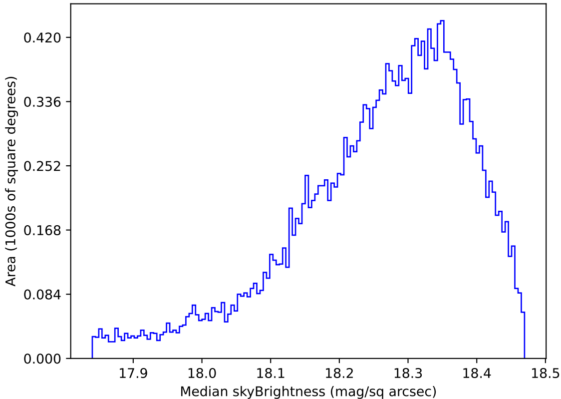
ddf_acor_sf30_lsf40_lsr10_v3.4_10yrs Yr 1 y band: Median skyBrightness
