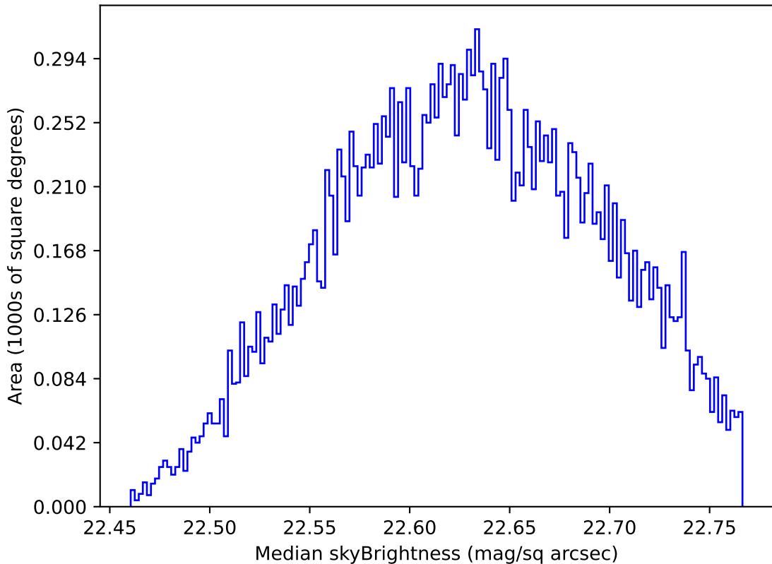
ddf_acor_sf30_lsf40_lsr10_v3.4_10yrs Yr 1 u band: Median skyBrightness
