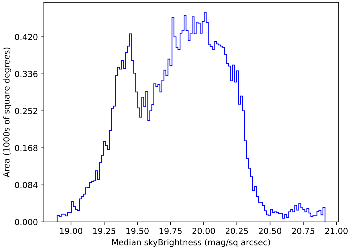
ddf_acor_sf30_lsf40_lsr10_v3.4_10yrs Yr 1 all bands: Median skyBrightness
