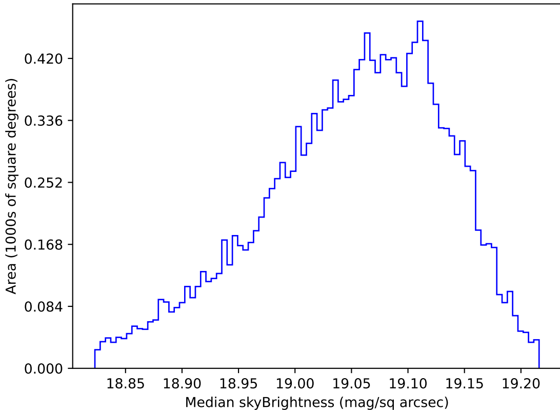
ddf_acor_sf30_lsf40_lsr10_v3.4_10yrs WFD z band: Median skyBrightness
