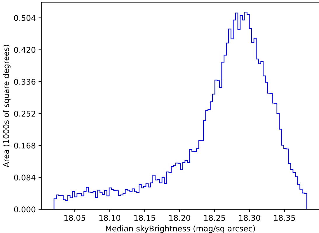
ddf_acor_sf30_lsf40_lsr10_v3.4_10yrs WFD y band: Median skyBrightness
