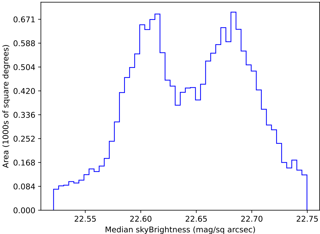
ddf_acor_sf30_lsf40_lsr10_v3.4_10yrs WFD u band: Median skyBrightness
