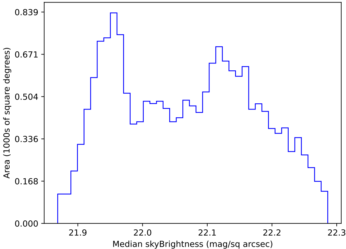
ddf_acor_sf30_lsf40_lsr10_v3.4_10yrs WFD g band: Median skyBrightness
