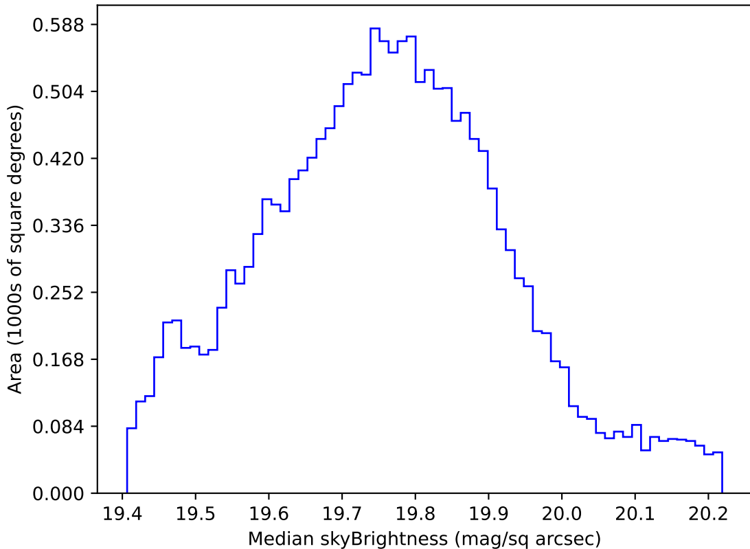
ddf_acor_sf30_lsf40_lsr10_v3.4_10yrs WFD all bands: Median skyBrightness
