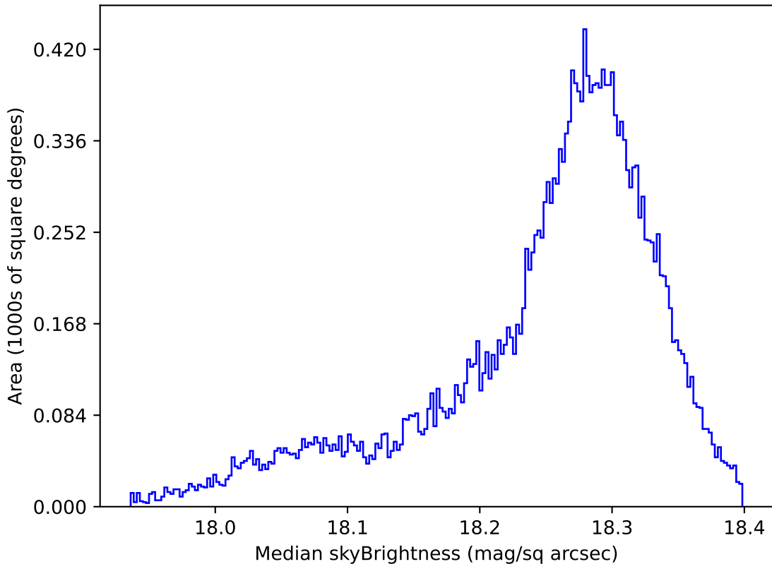
ddf_acor_sf30_lsf40_lsr10_v3.4_10yrs All sky y band: Median skyBrightness
