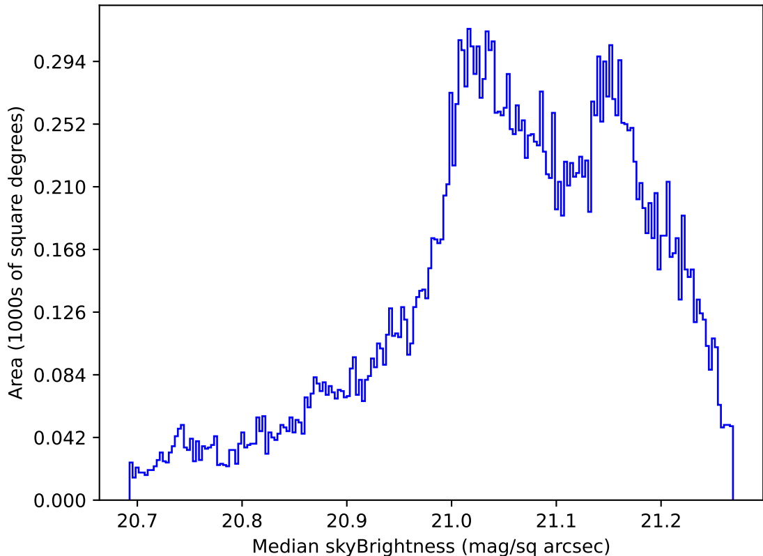
ddf_acor_sf30_lsf40_lsr10_v3.4_10yrs All sky r band: Median skyBrightness
