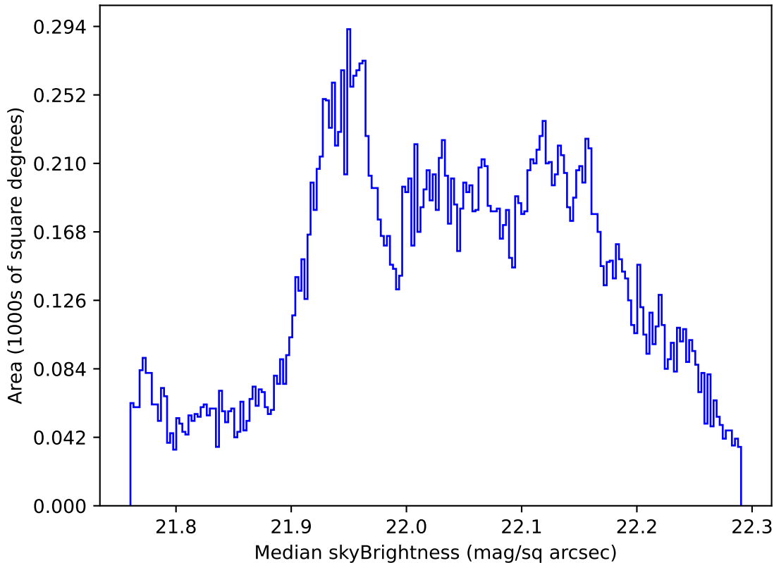
ddf_acor_sf30_lsf40_lsr10_v3.4_10yrs All sky g band: Median skyBrightness
