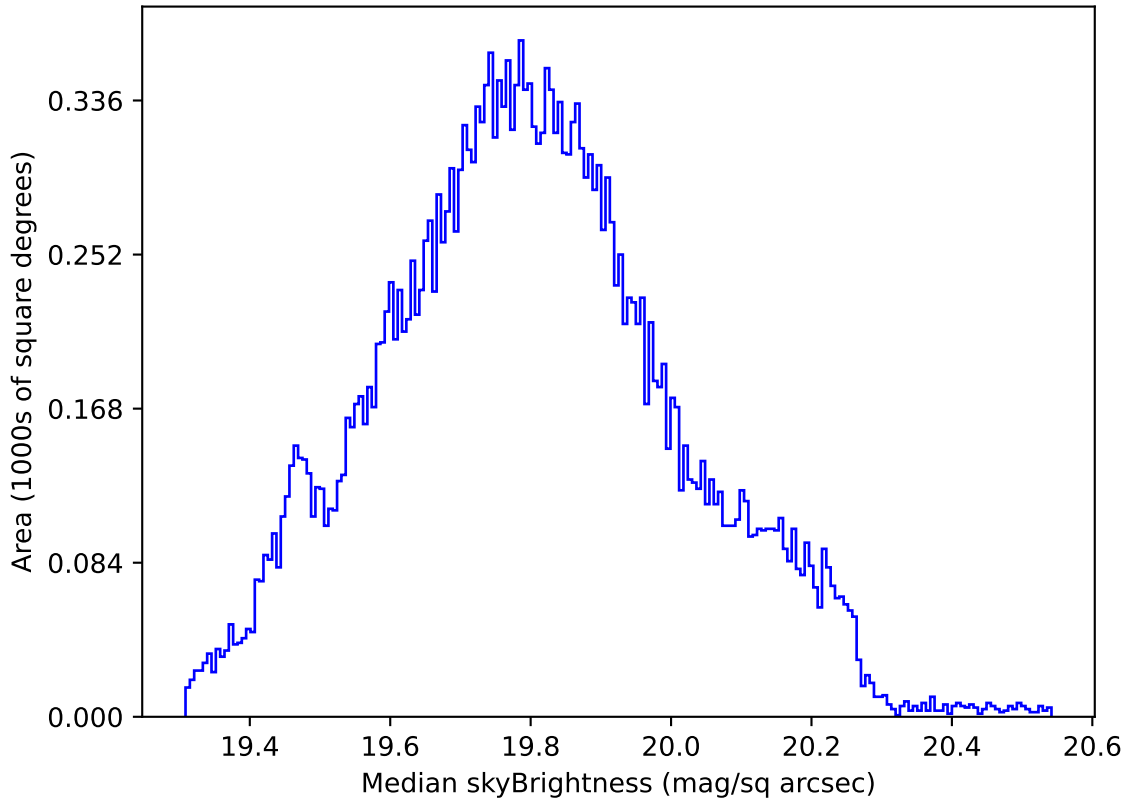
ddf_acor_sf30_lsf40_lsr10_v3.4_10yrs All sky all bands: Median skyBrightness
