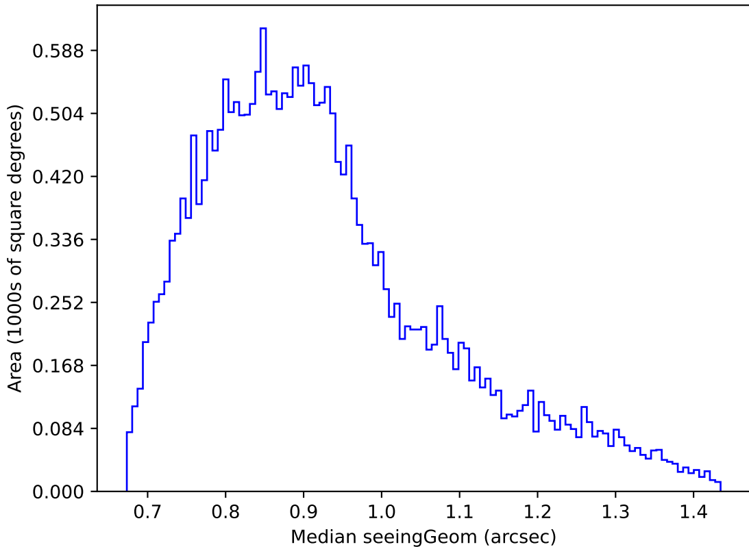
ddf_acor_sf30_lsf40_lsr10_v3.4_10yrs Yr 1 g band: Median seeingGeom
