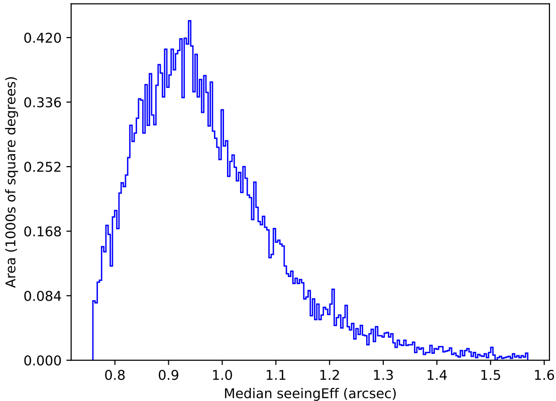
ddf_acor_sf30_lsf40_lsr10_v3.4_10yrs Yr 1 z band: Median seeingEff
