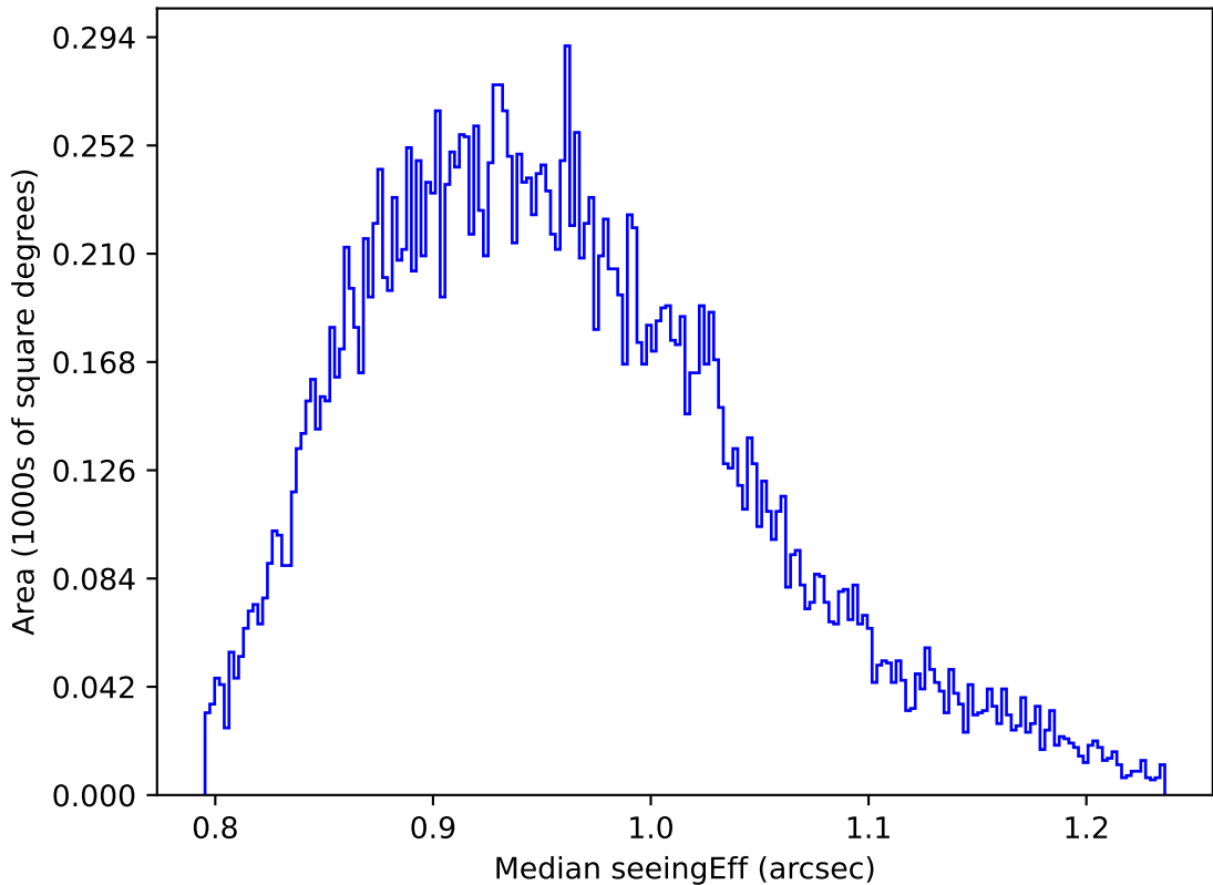
ddf_acor_sf30_lsf40_lsr10_v3.4_10yrs Yr 1 y band: Median seeingEff
