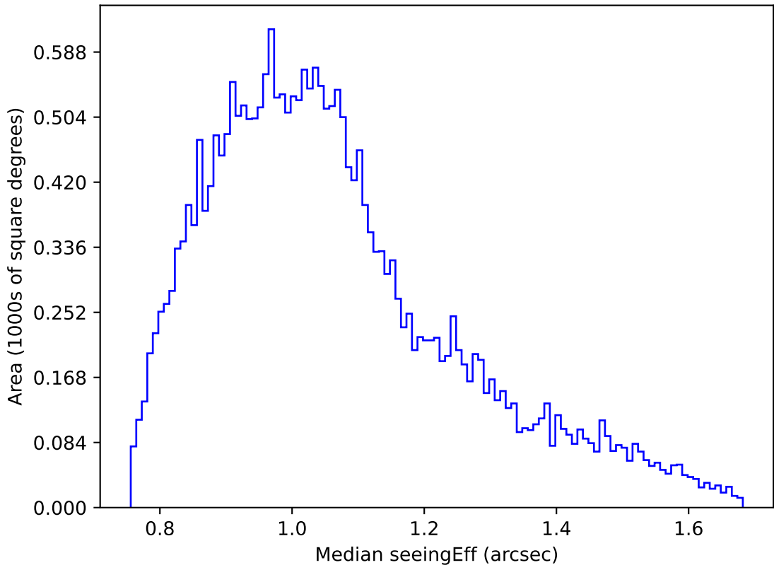
ddf_acor_sf30_lsf40_lsr10_v3.4_10yrs Yr 1 g band: Median seeingEff
