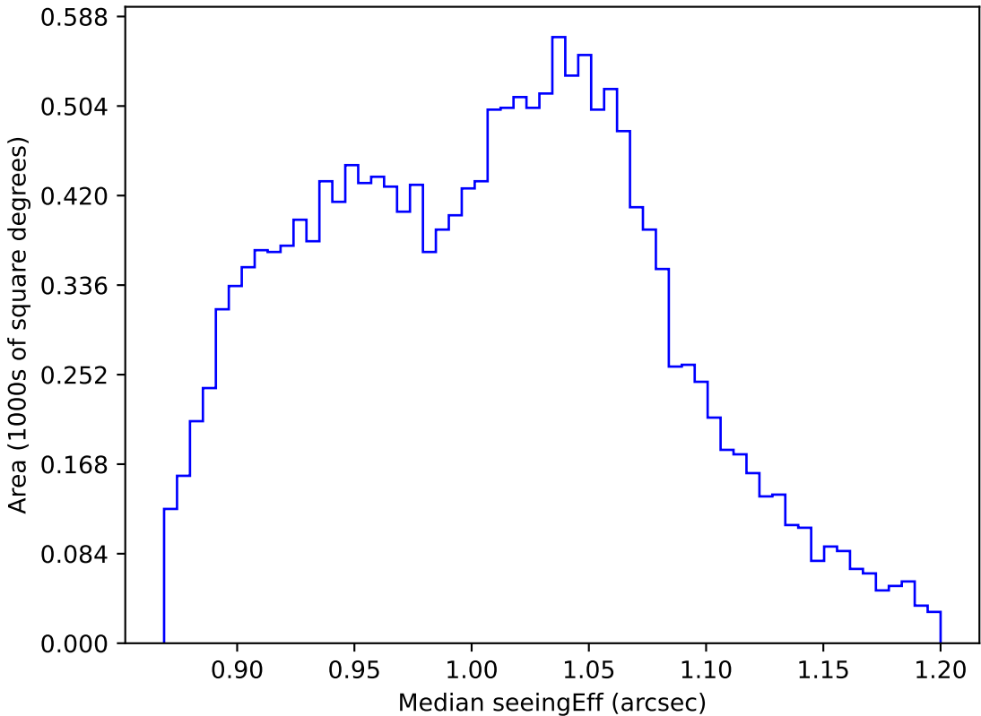
ddf_acor_sf30_lsf40_lsr10_v3.4_10yrs WFD z band: Median seeingEff
