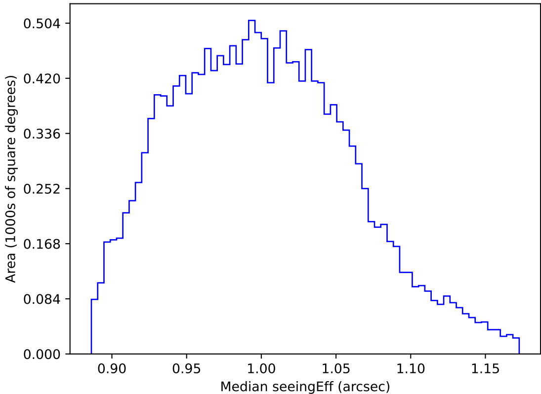
ddf_acor_sf30_lsf40_lsr10_v3.4_10yrs WFD y band: Median seeingEff
