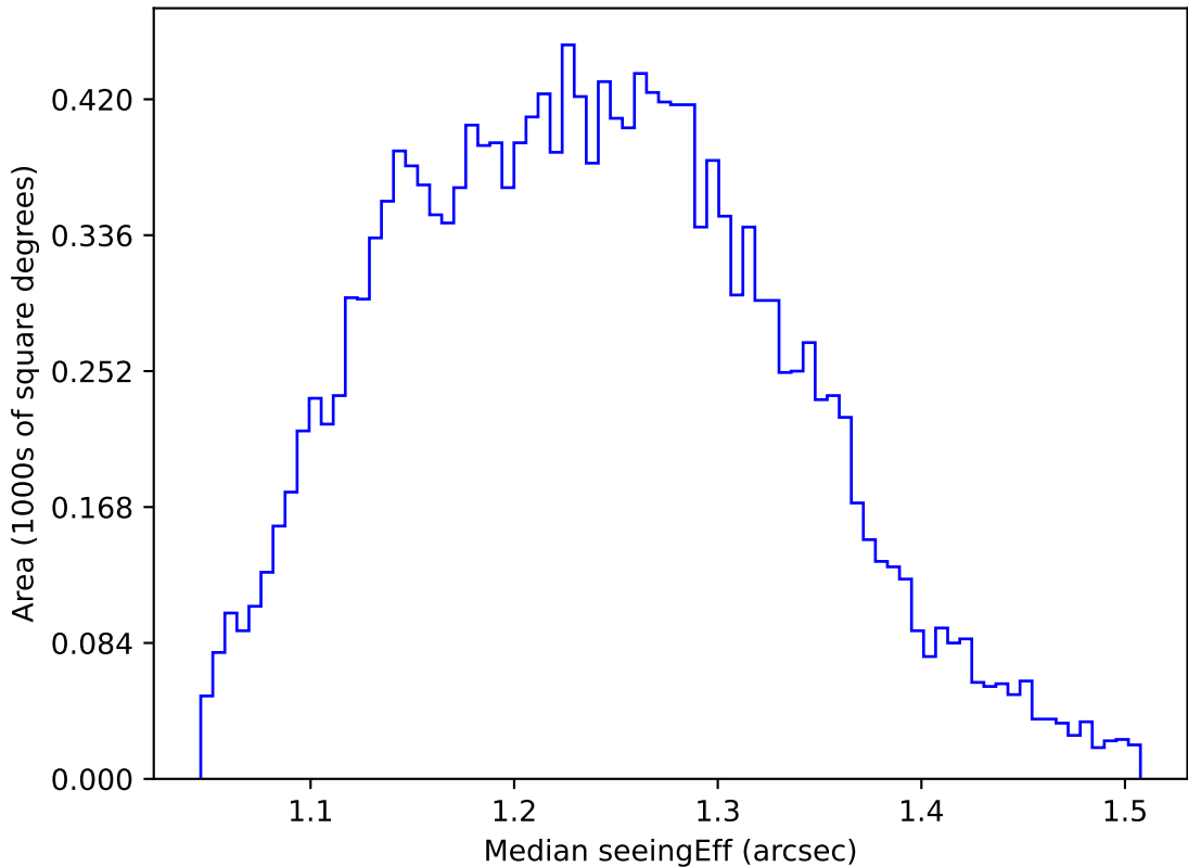
ddf_acor_sf30_lsf40_lsr10_v3.4_10yrs WFD u band: Median seeingEff
