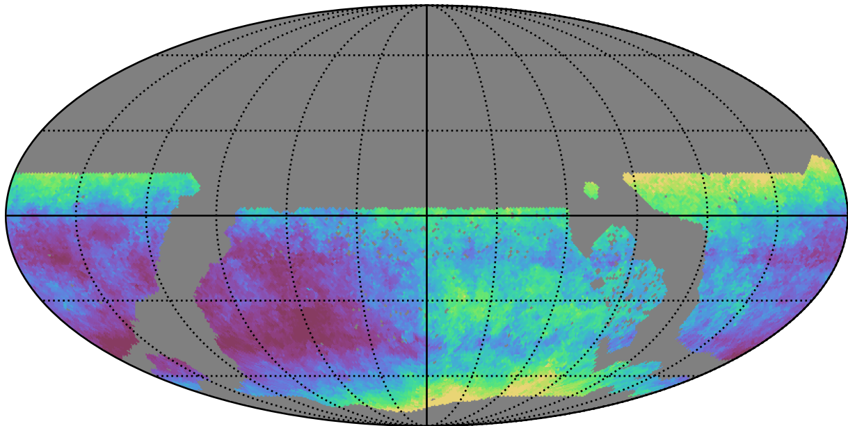
ddf_acor_sf30_lsf40_lsr10_v3.4_10yrs WFD i band: Median seeingEff
