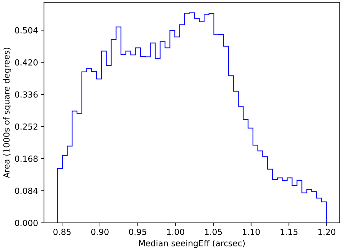
ddf_acor_sf30_lsf40_lsr10_v3.4_10yrs WFD i band: Median seeingEff
