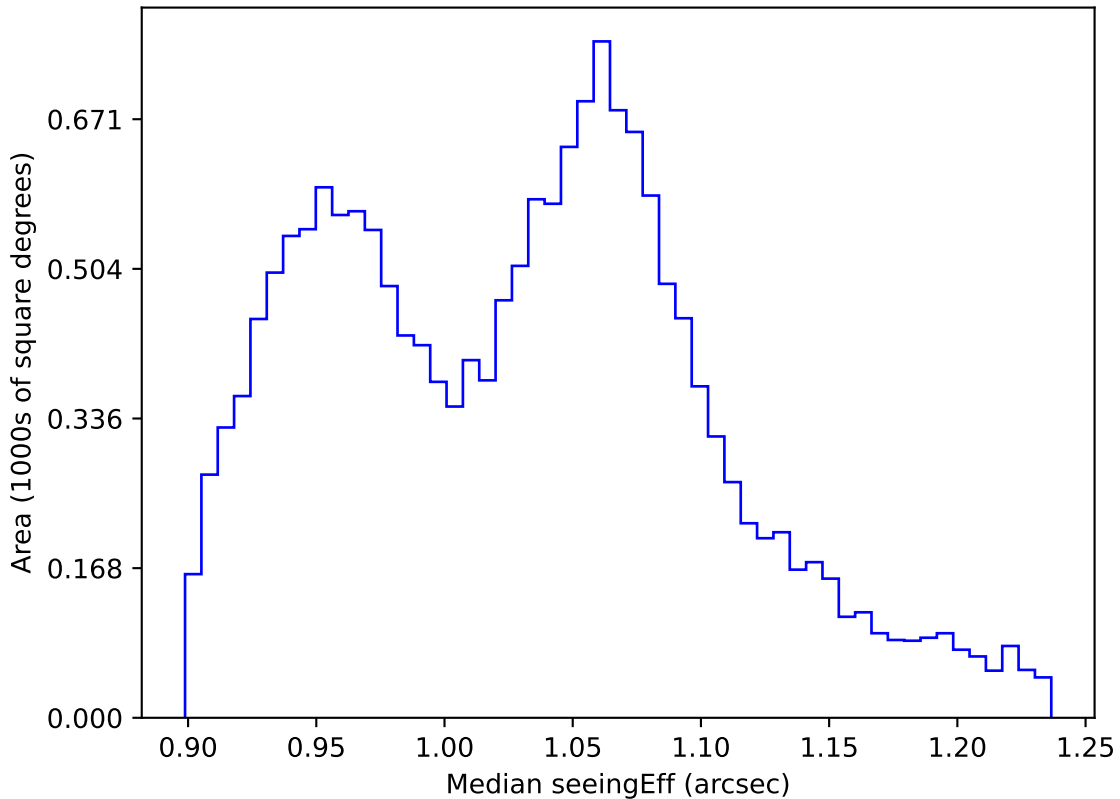
ddf_acor_sf30_lsf40_lsr10_v3.4_10yrs WFD all bands: Median seeingEff
