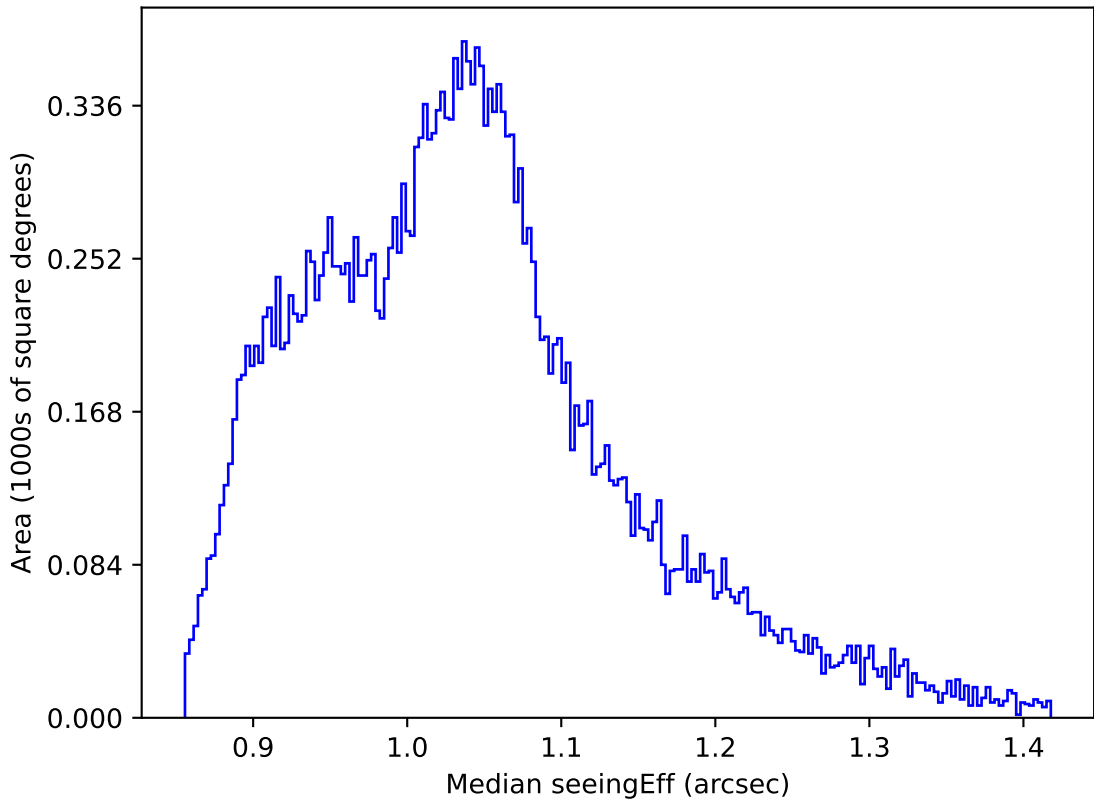
ddf_acor_sf30_lsf40_lsr10_v3.4_10yrs All sky z band: Median seeingEff
