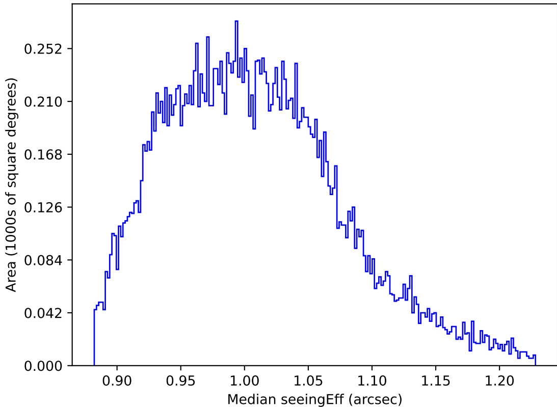
ddf_acor_sf30_lsf40_lsr10_v3.4_10yrs All sky y band: Median seeingEff
