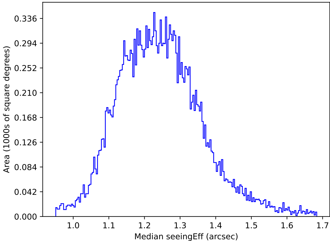
ddf_acor_sf30_lsf40_lsr10_v3.4_10yrs All sky u band: Median seeingEff
