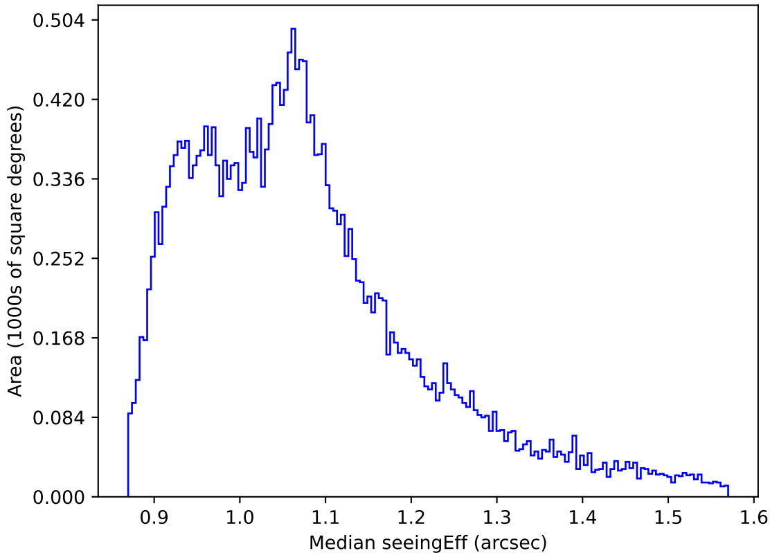
ddf_acor_sf30_lsf40_lsr10_v3.4_10yrs All sky r band: Median seeingEff
